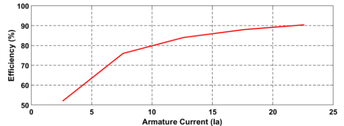
Fig. 10. Proposed DC Motor Armature Current Vs Efficiency
