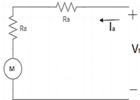
Fig. 5. Series Motor Equivalent Circuit
