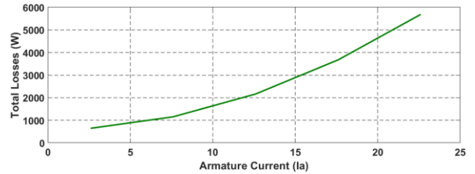
Fig. 7. Typical DC Motor Armature Current Vs Losses
