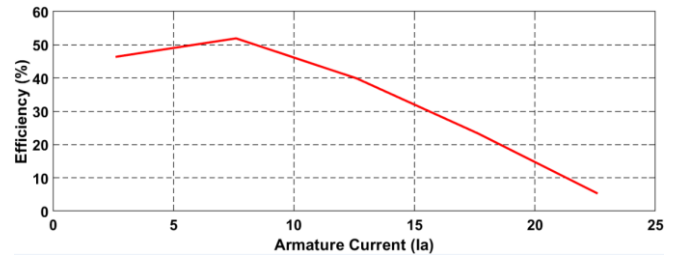
Fig. 8. Typical DC Motor Armature Current Vs Efficiency
